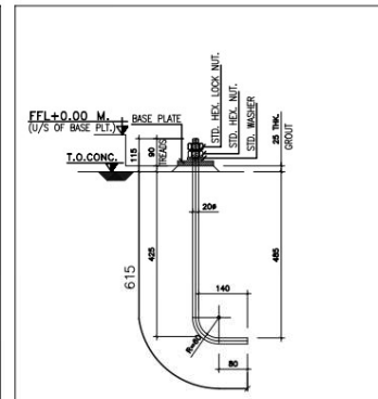
M-20 ANCHOR BOLT DETAIL (16 Nos. REQD.)
