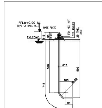
M-24 ANCHOR BOLT DETAIL (56 Nos. REQD.)
