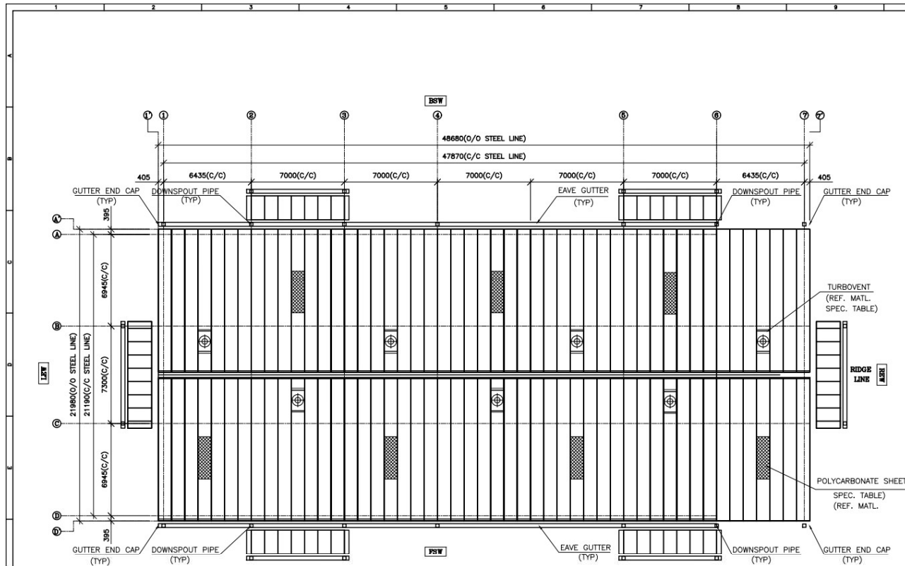
ROOF SHEETING PLAN
