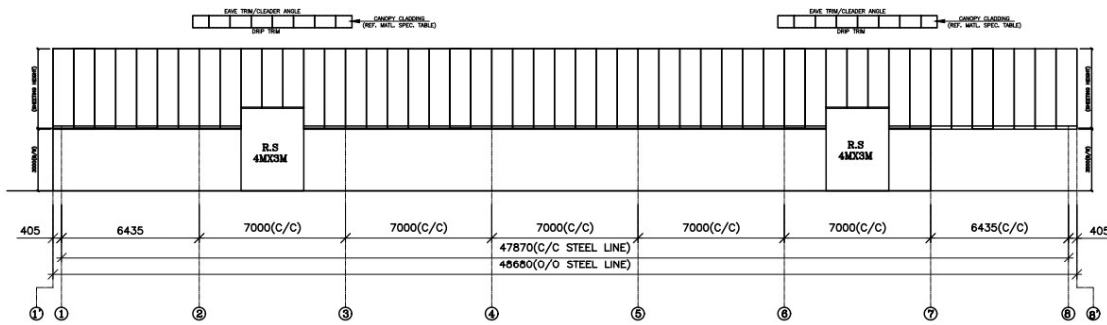
SHEETING ELEVATION PLAN (FOR GRID LINE A)
