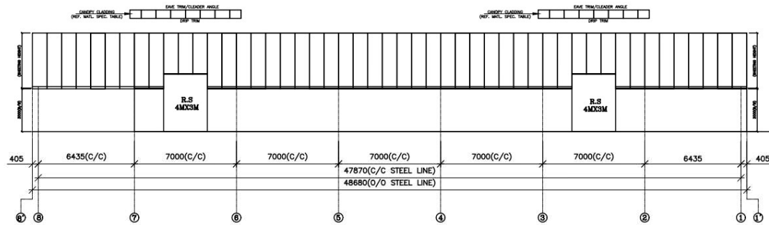
SHEETING ELEVATION PLAN (FOR GRID LINE D)
