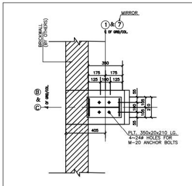
DETAIL D3 (AS DRAWN) (2 No. REQD.) GA-01 DETAIL D3X (OPP. HAND) (2 No. REQD.) GA-01
